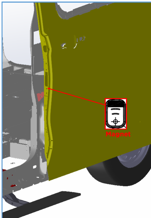
Detail Türsensor
